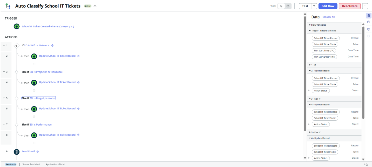
Figure 1: Published Auto Classify School IT Tickets Flow Designer workflow.
